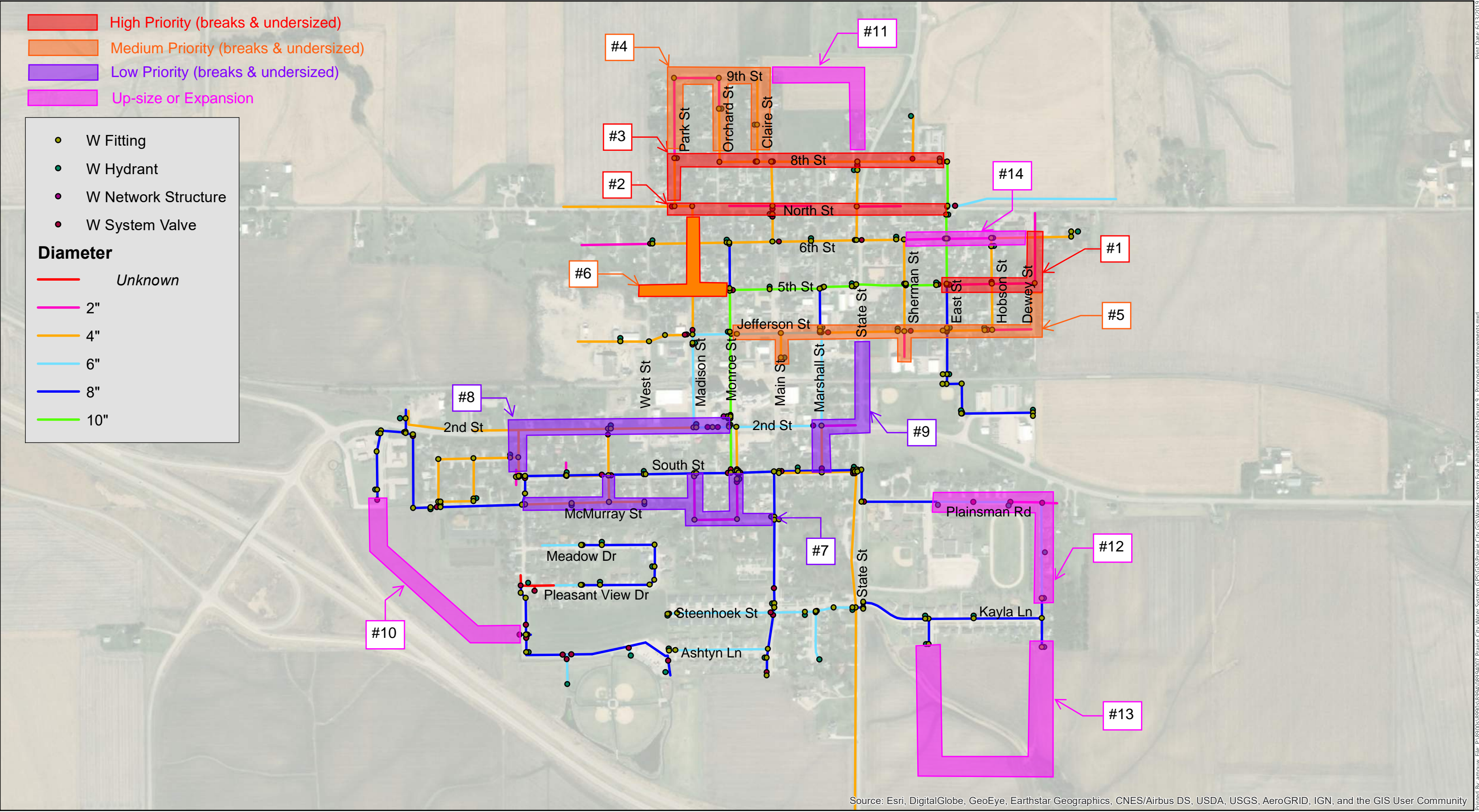
Figure 6 - Proposed Water System Improvements
